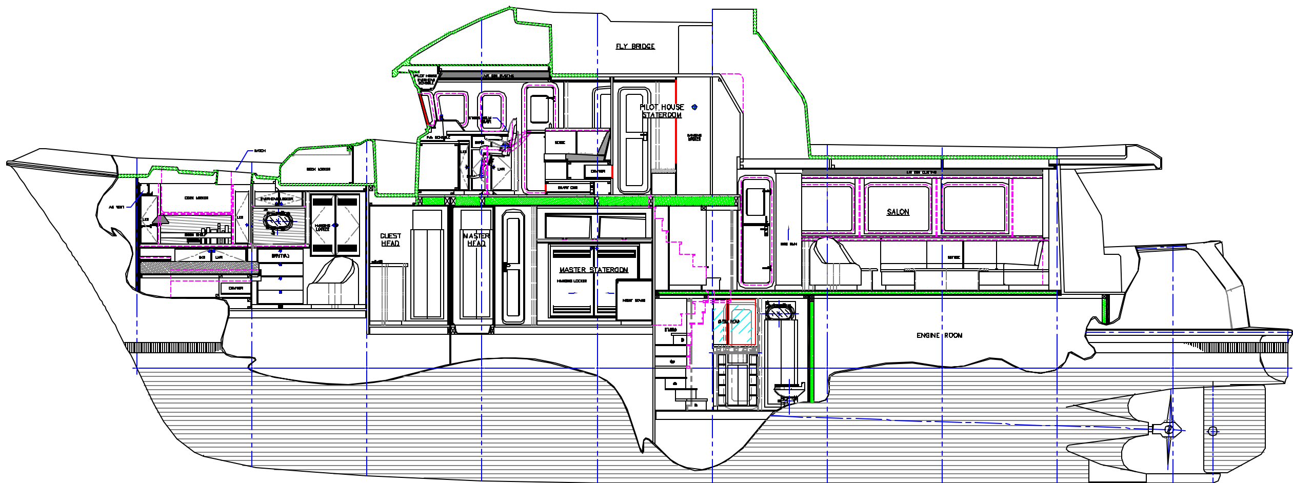
STARBOARD INTERIOR PROFILE SECTION 1/2-1-1
